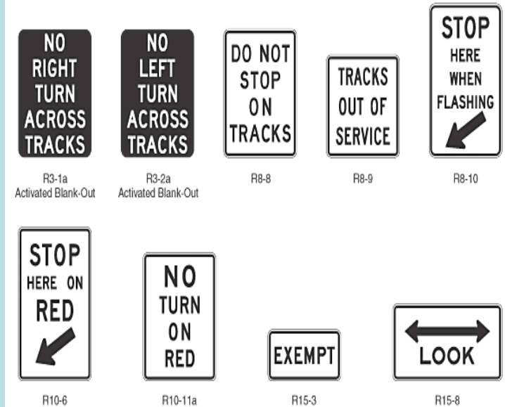
Figure 8B-3. Regulatory Signs
